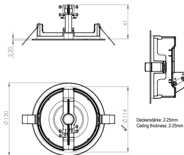
Dimensions recessed frame NLILDE (mm)
