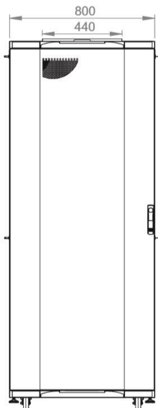
Front view
