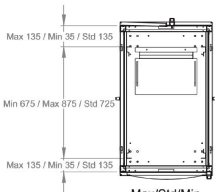
Max/Std/Min Equipment mounting distance
