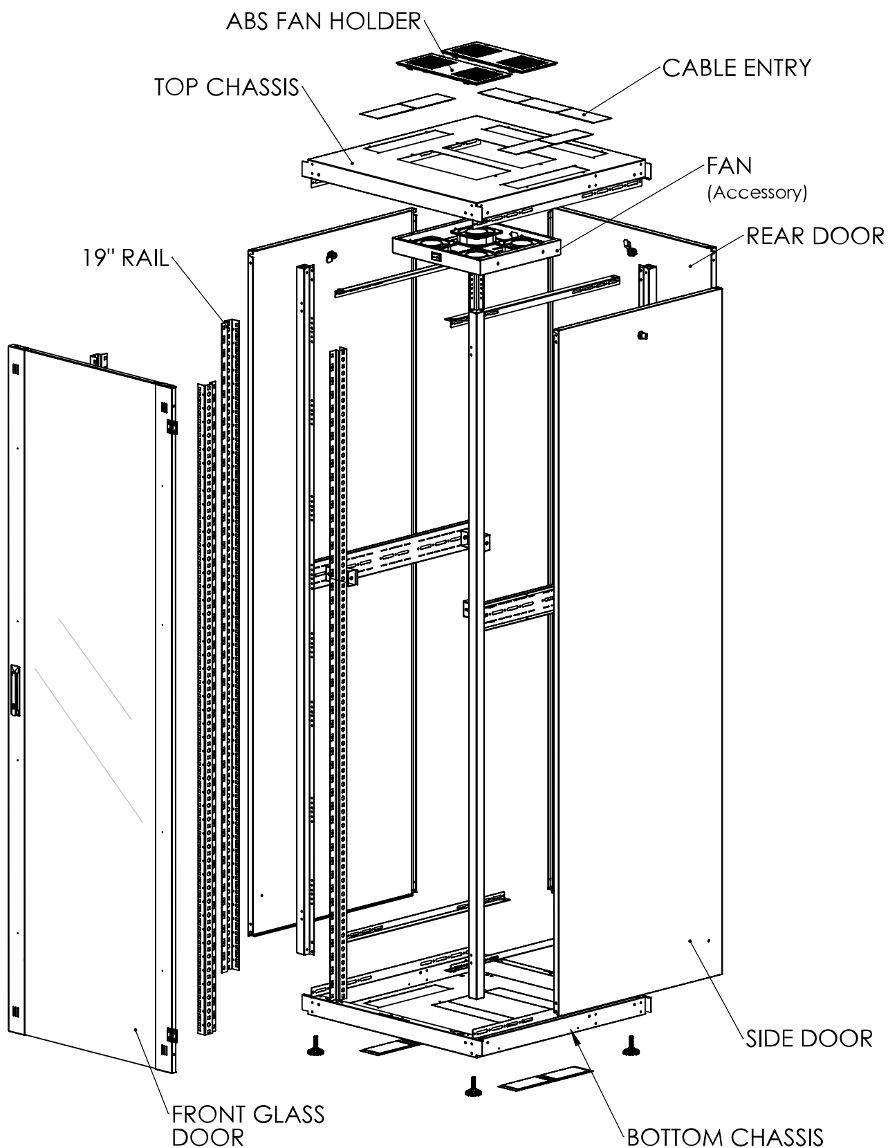
Exploded view
