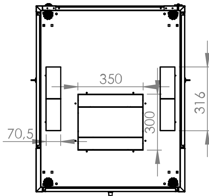
Bottom view
